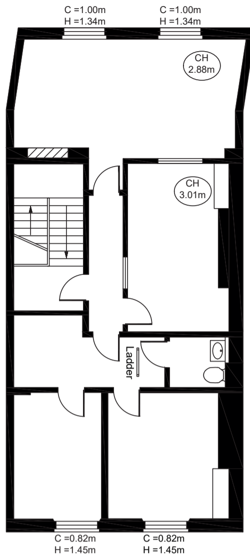
Second Floor Approximate Gross Internal Area 72.37 sq m / 779 sq ft
